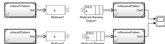
Run based on message availability
