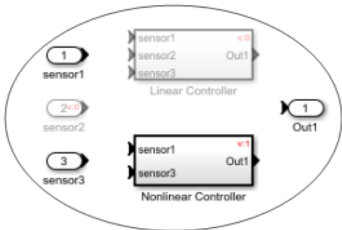
Components of 'Controller' block
